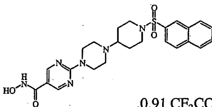
.091 CF 3 COOH compound 3
